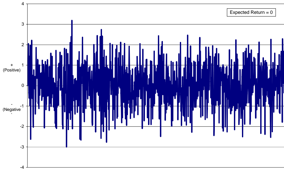
White Noise
