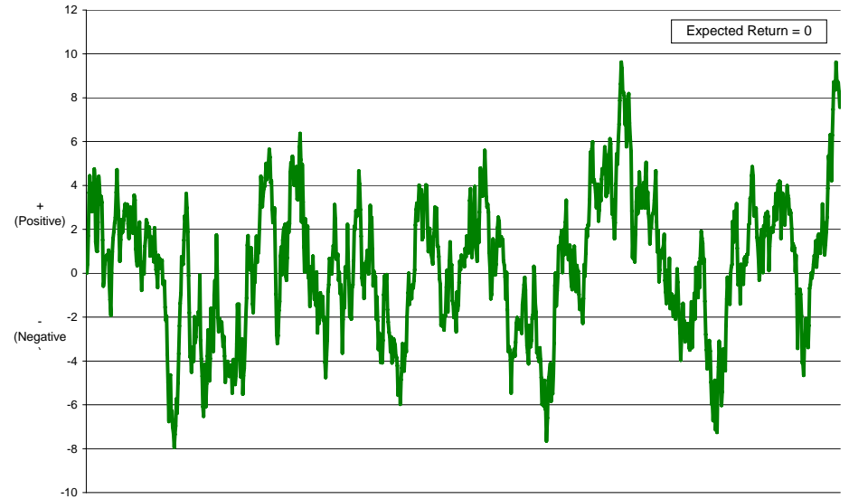
Random Walk
