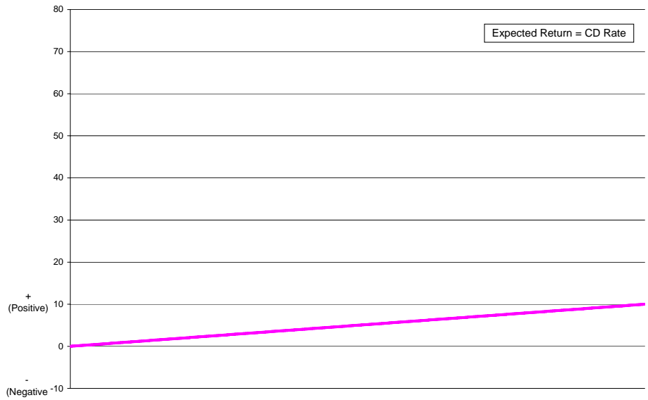
Deterministic
